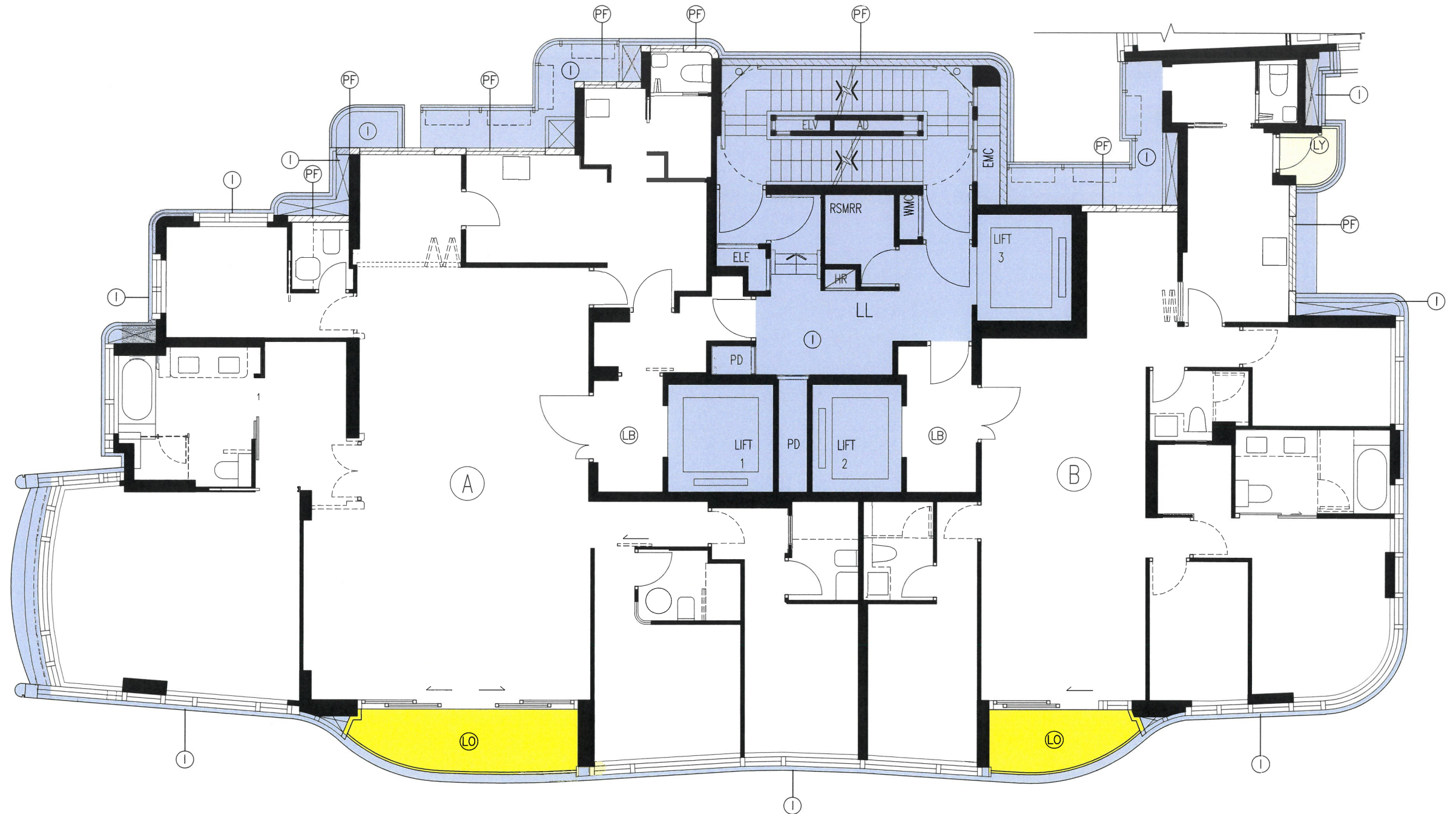
TOWER 1 22/F (HIGH ZONE) PLAN
