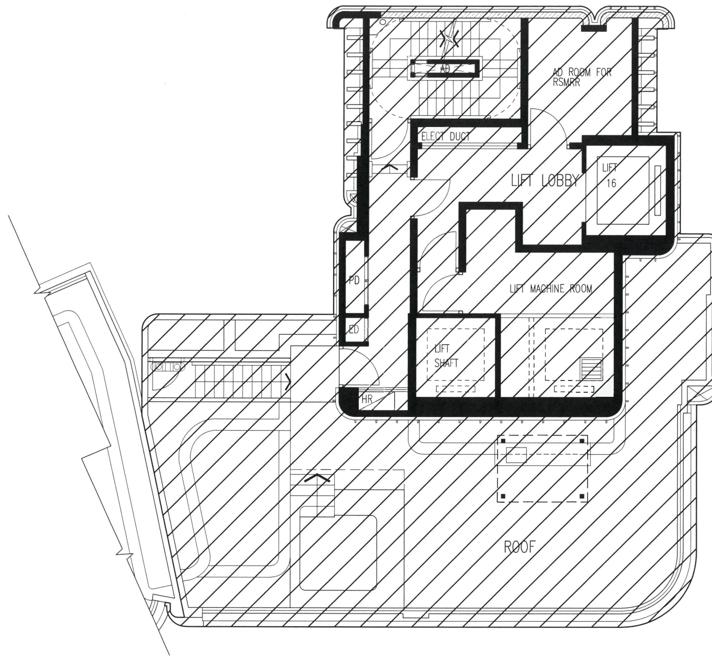
TOWER 7 MAIN ROOF PLAN
