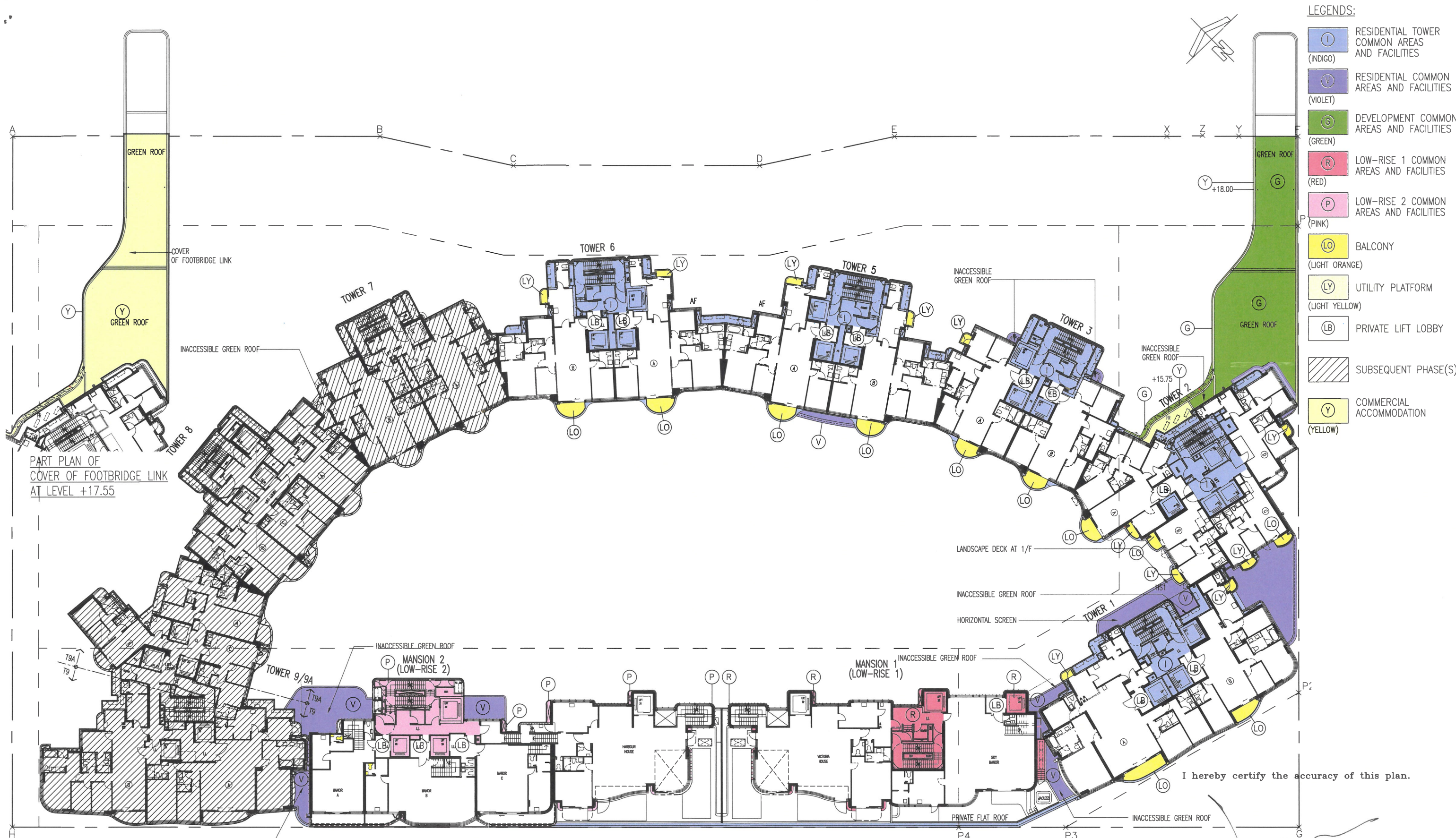
SECOND FLOOR PLAN (TOWER No. 4 NOT USED)
