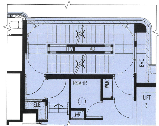
TOWER 1 2/F PART PLAN
