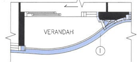
TOWER 1 25/F PART PLAN
