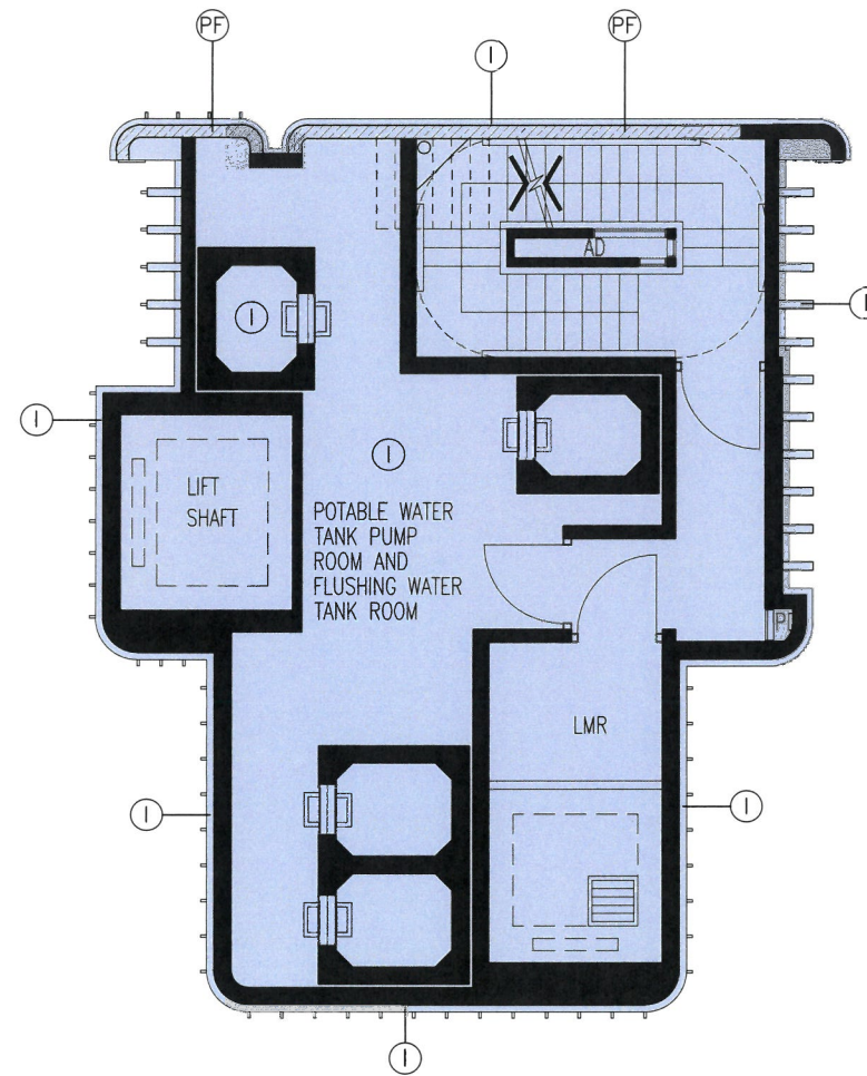
TOWER 3 INTERMEDIATE ROOF PLAN
