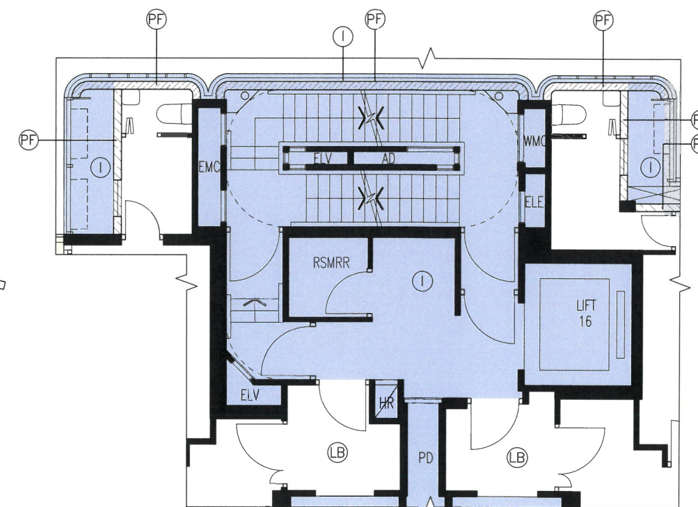
TOWER 6 2/F PART PLAN
