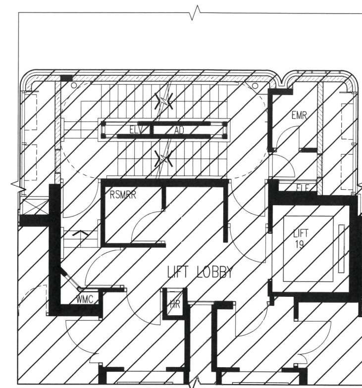
TOWER 7 2/F PART PLAN
