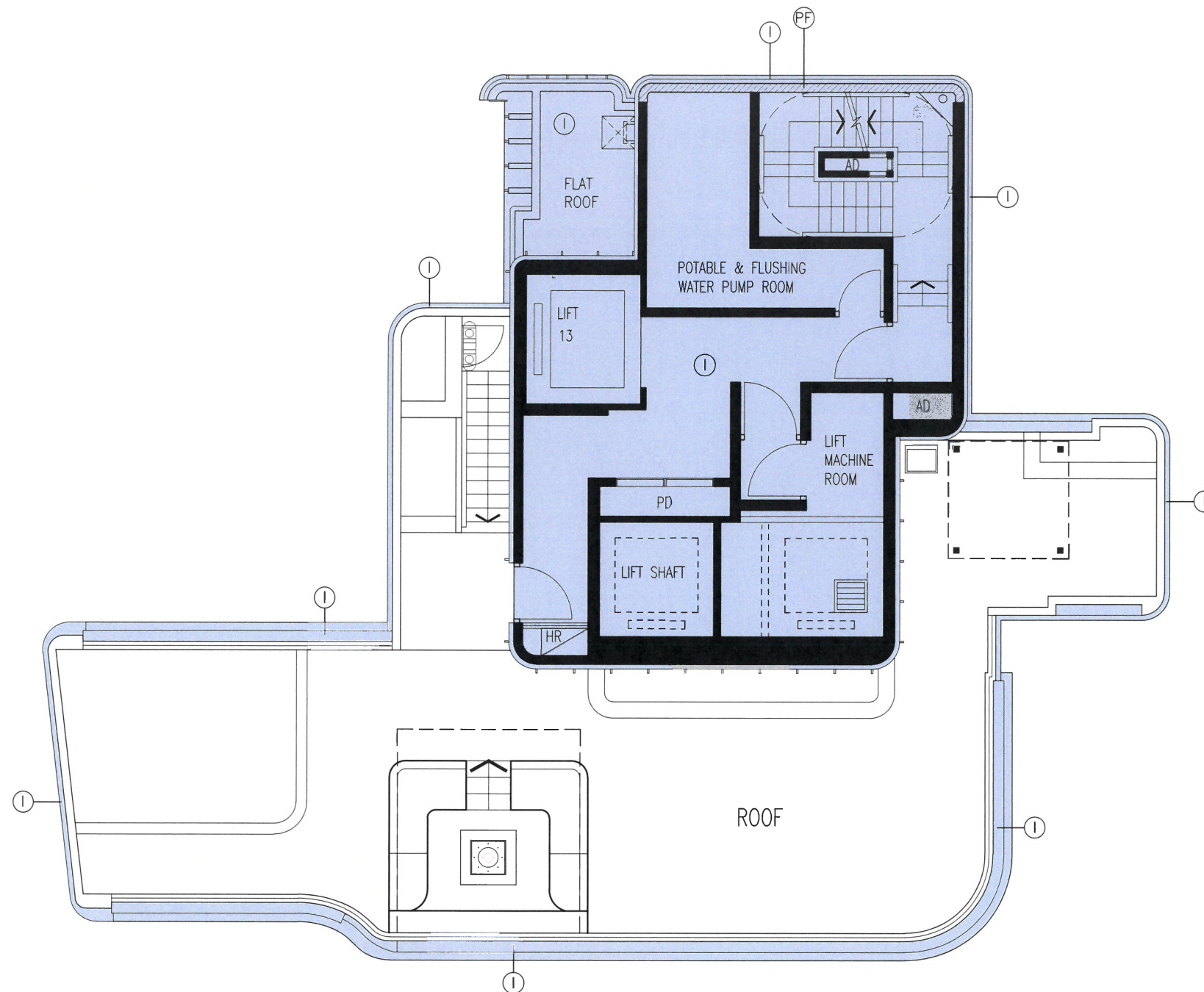
TOWER 5 MAIN ROOF PLAN
