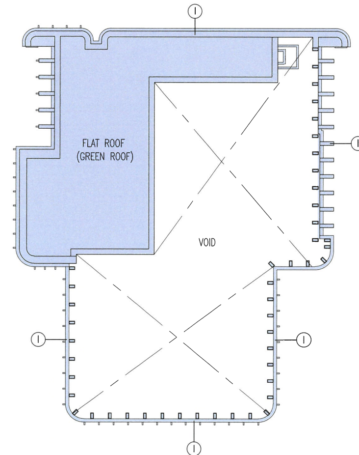
TOWER 3 TOP ROOF PLAN
