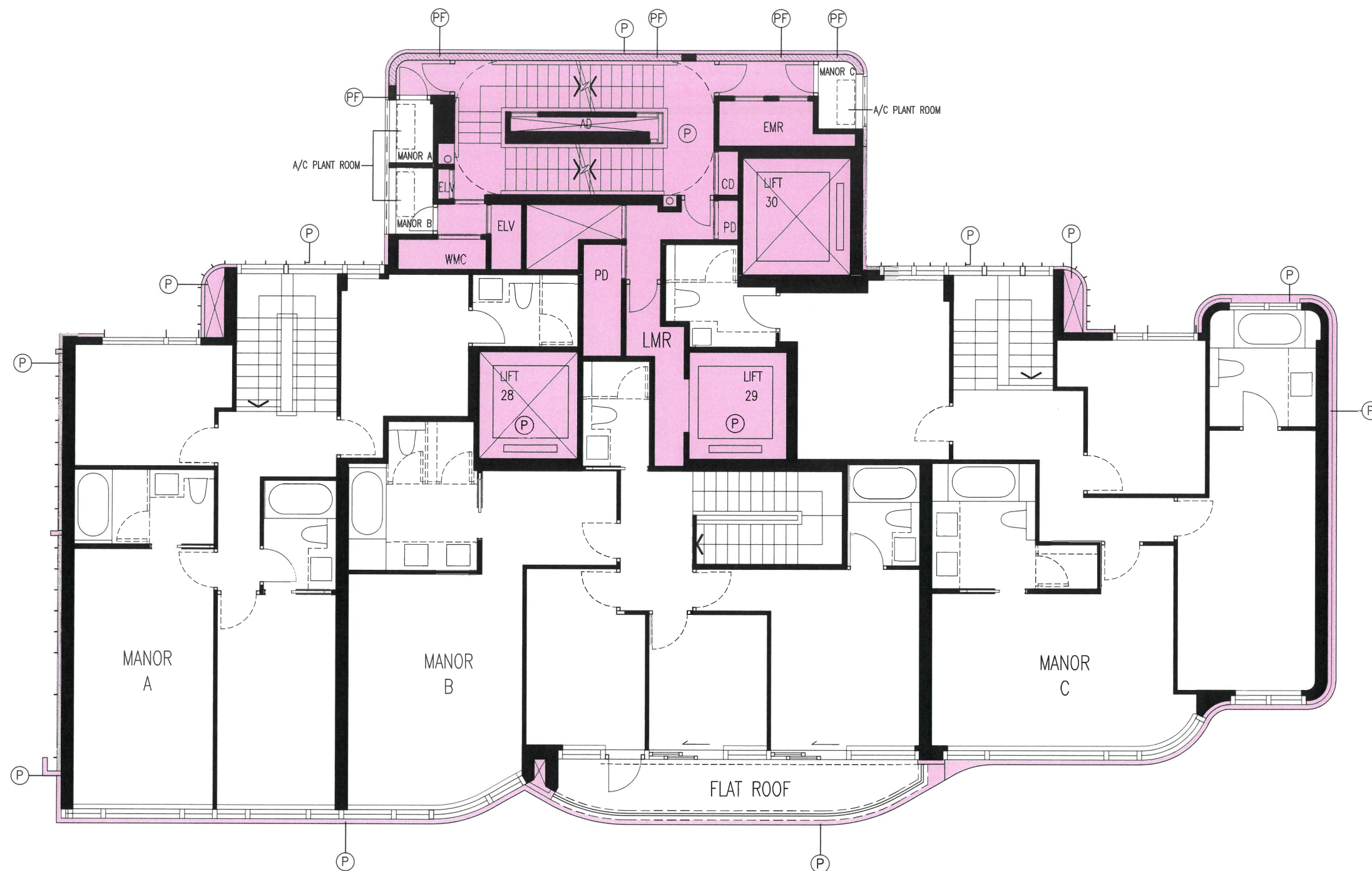
MANSION 2 (LOW-RISE 2) 6/F PLAN (UPPER DUPLEX)
