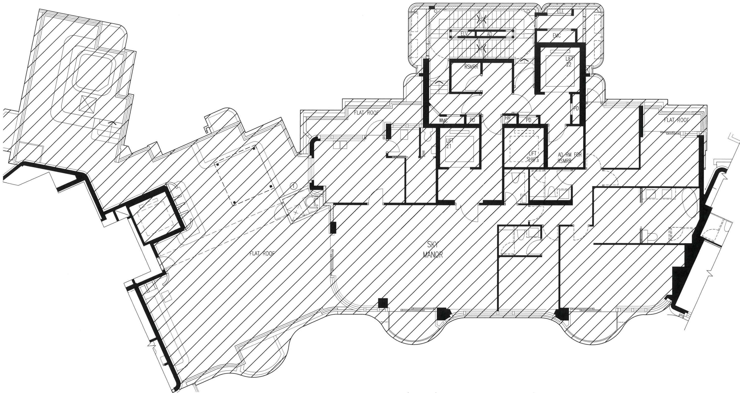
TOWER 8 27/F (LOWER SIMPLEX) PLAN
